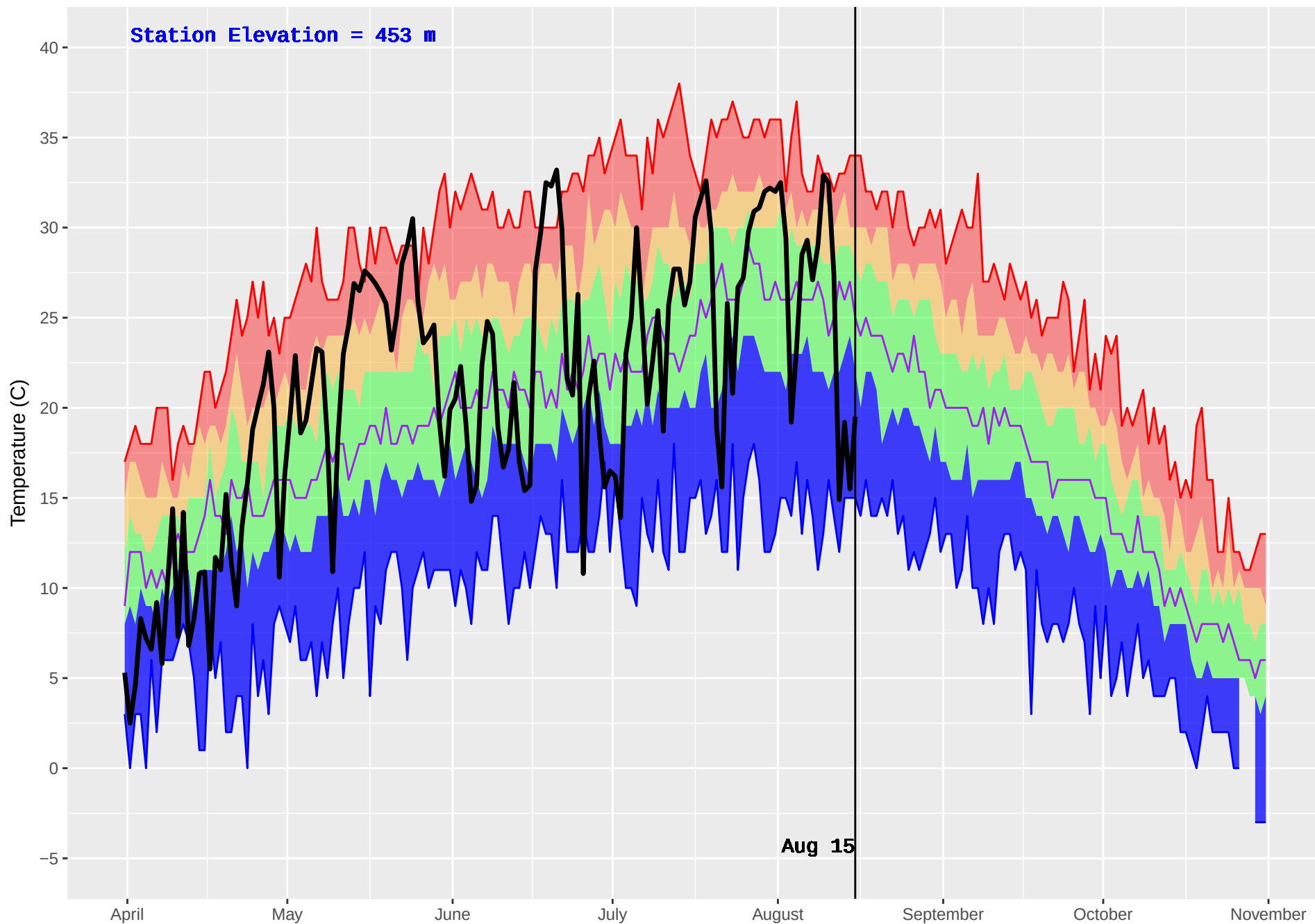
CLEARWATER HUB (239) : Historical (1976–2016) and Current (2018) Daily Temperature
