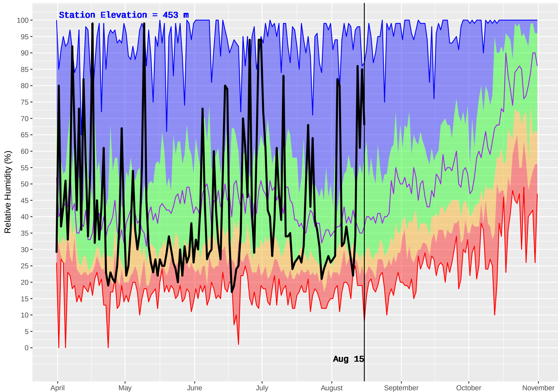
CLEARWATER HUB (239) : Historical (1976–2016) and Current (2018) Daily Relative Humidity
